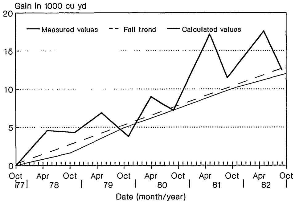
Figure 47. Volume change, October 1977-December 1982
