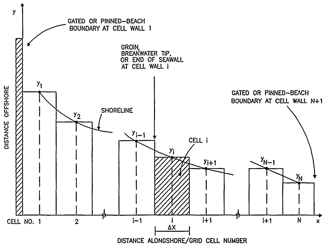
Figure 19. Example of a coordinate system and grid used by GENESIS
