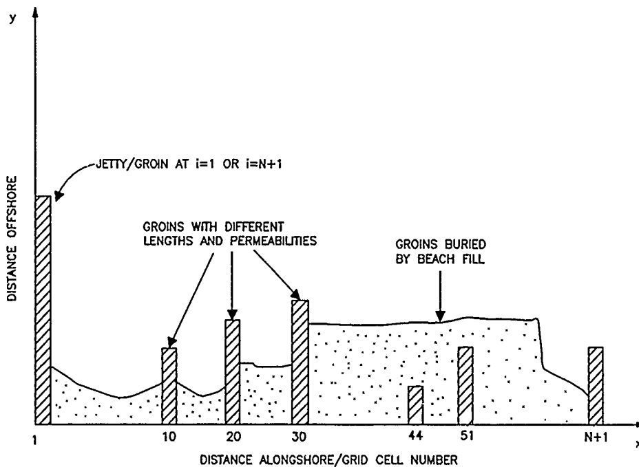
Figure 33. Legal placement of simple groins
