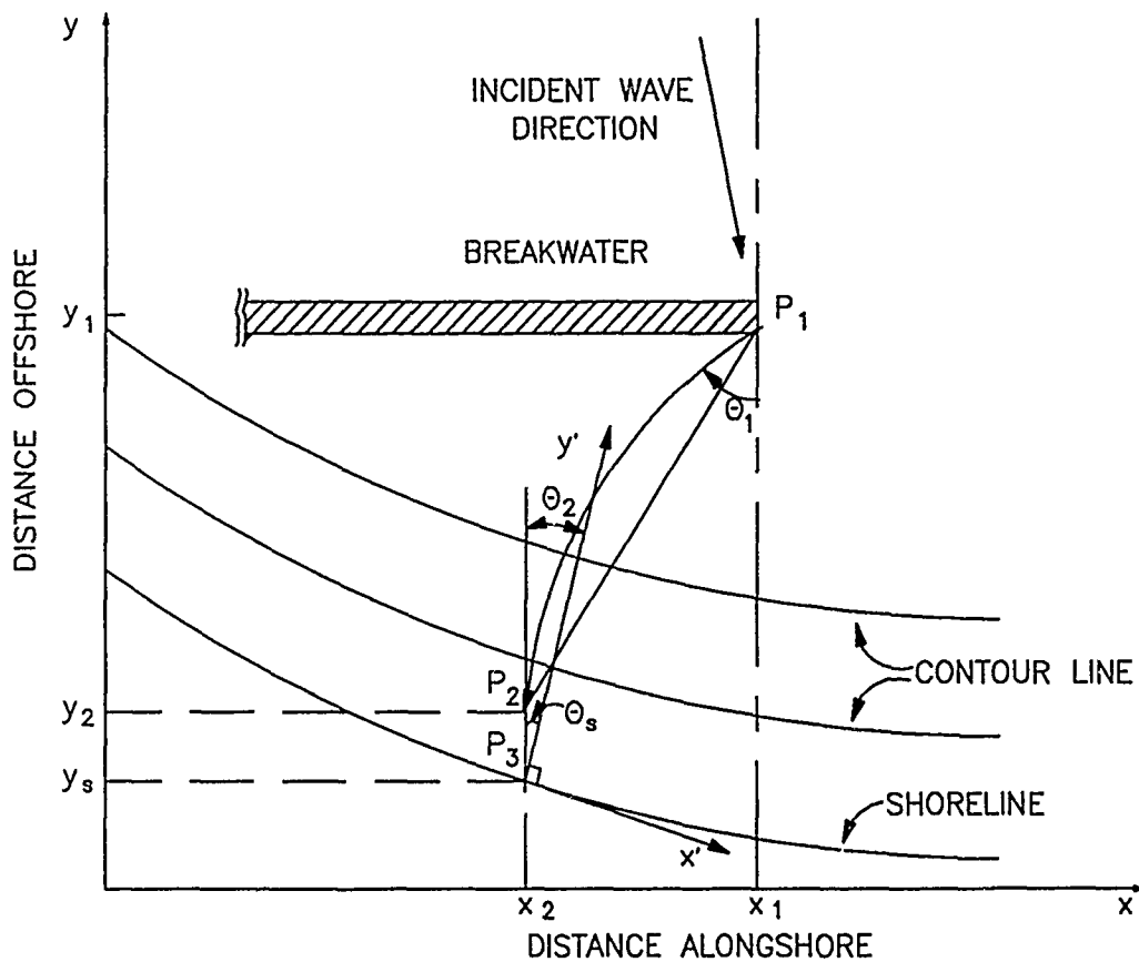
Figure 12. Wave angles in contour modification
