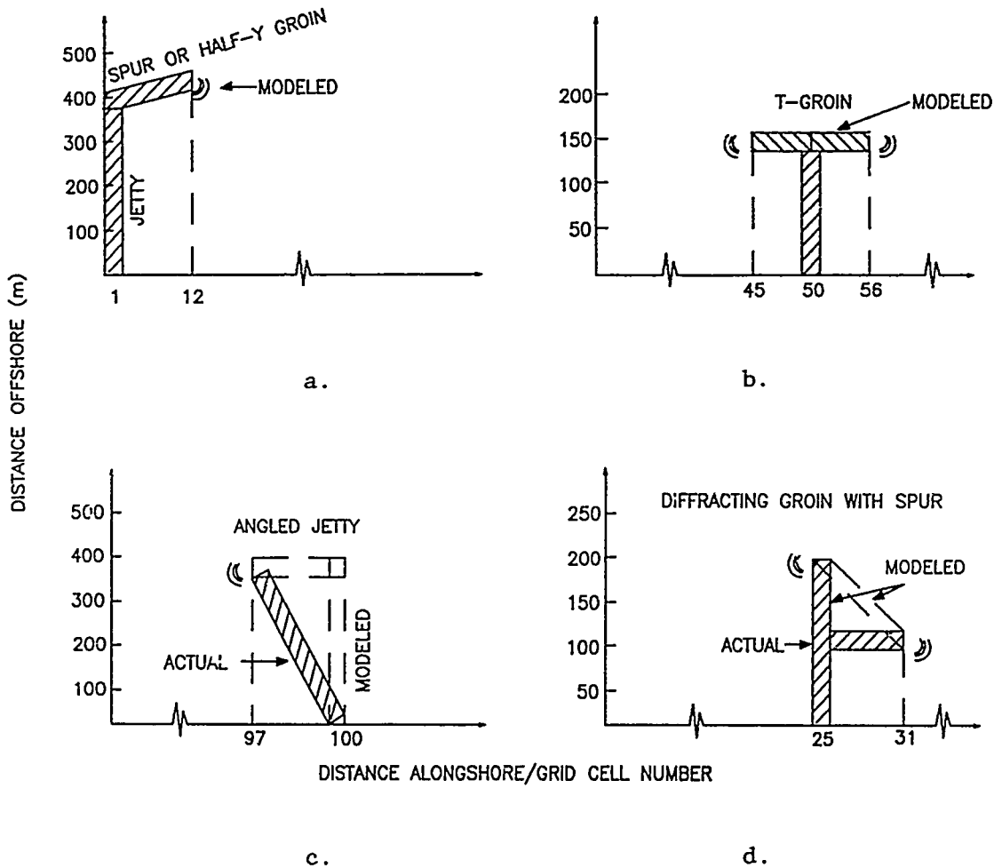
Figure 34. Examples of complex groin and jetty configurations
