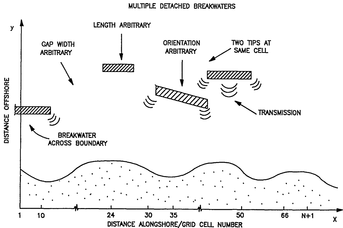
Figure 32. Parameters associated with detached breakwaters
