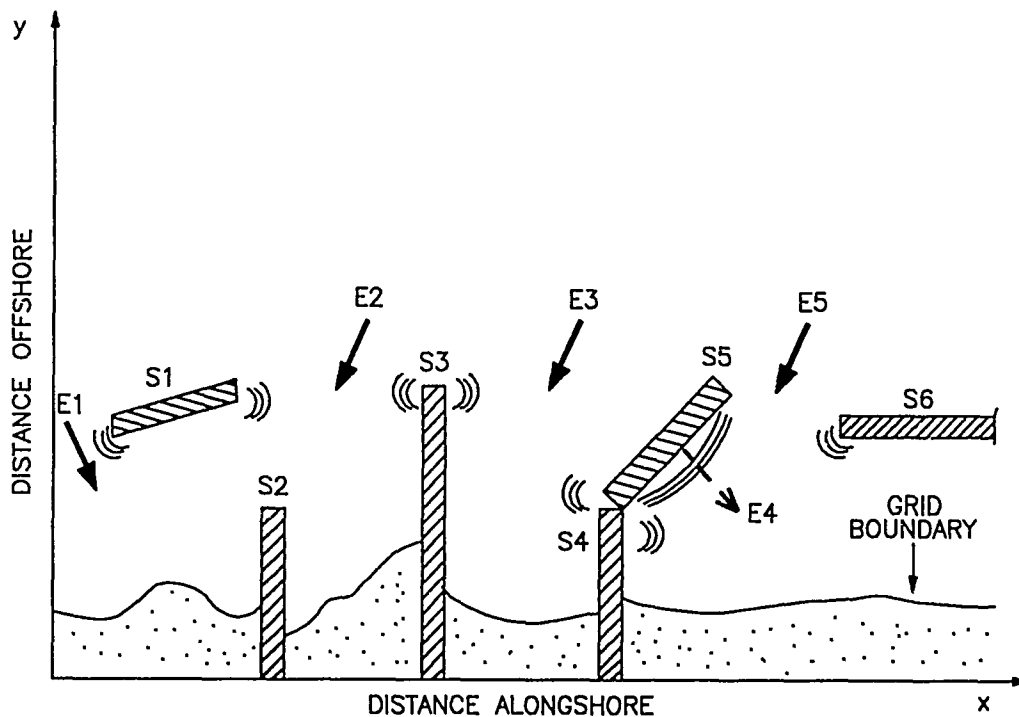
Figure 16. Energy windows and transport calculation domains
