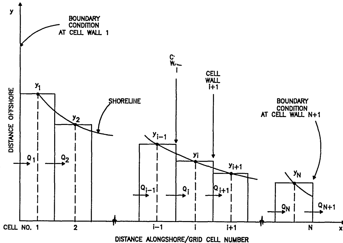
Figure 18. Finite difference staggered grid
