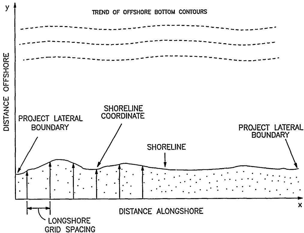
Figure 5. Model coordinate system
