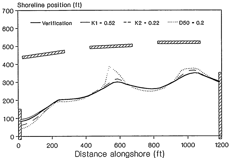
Figure 44. Model sensitivity to changes in K_1 , K_2 , and D_{50}
