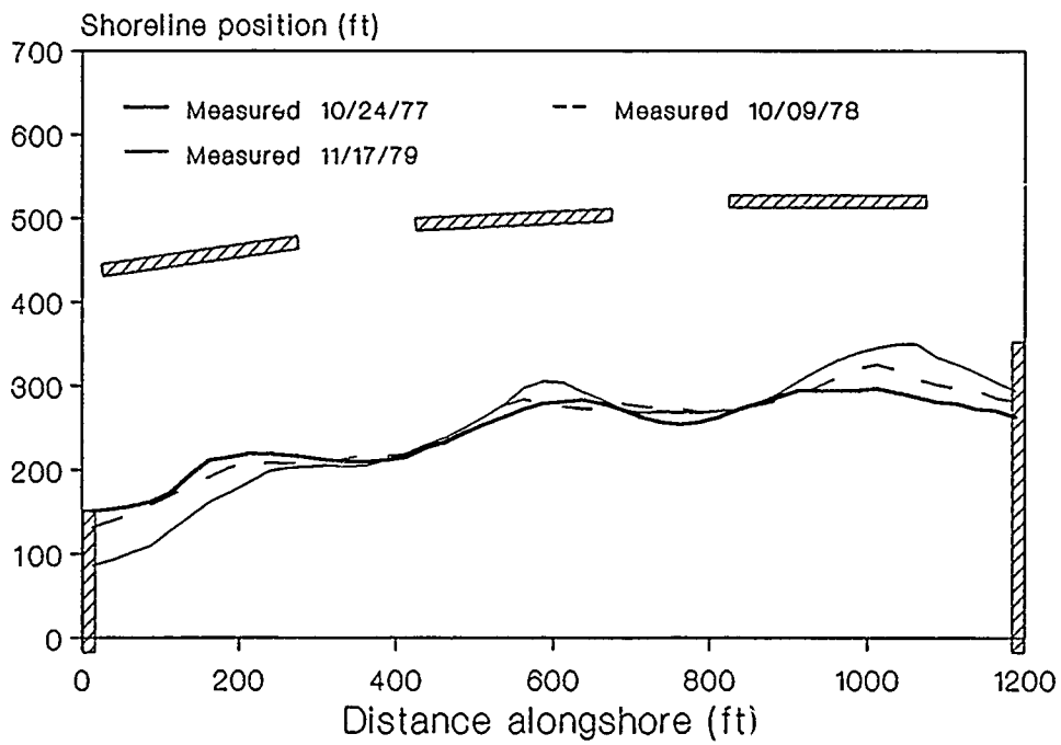
Figure 40. Adjusted measured shoreline positions
