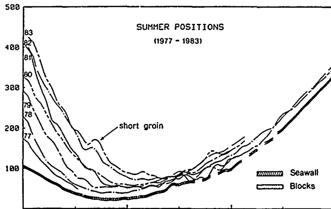
a. Summer shoreline positions
