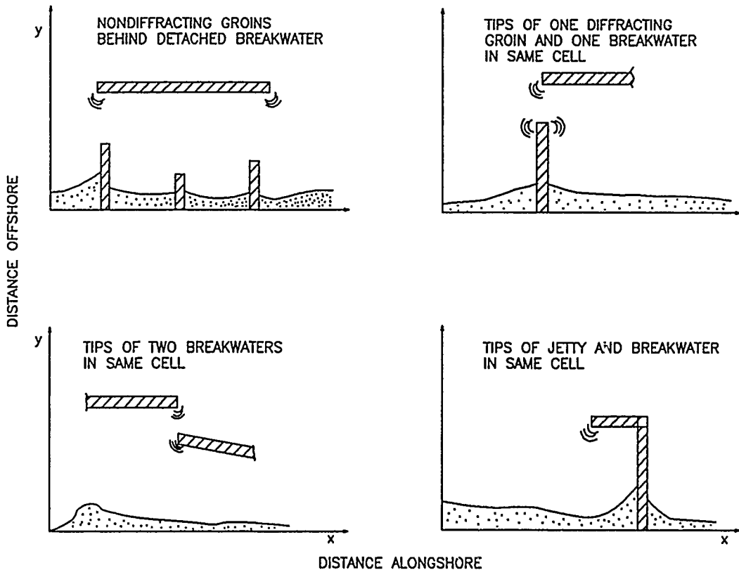
Figure 30. Example legal structure placements
