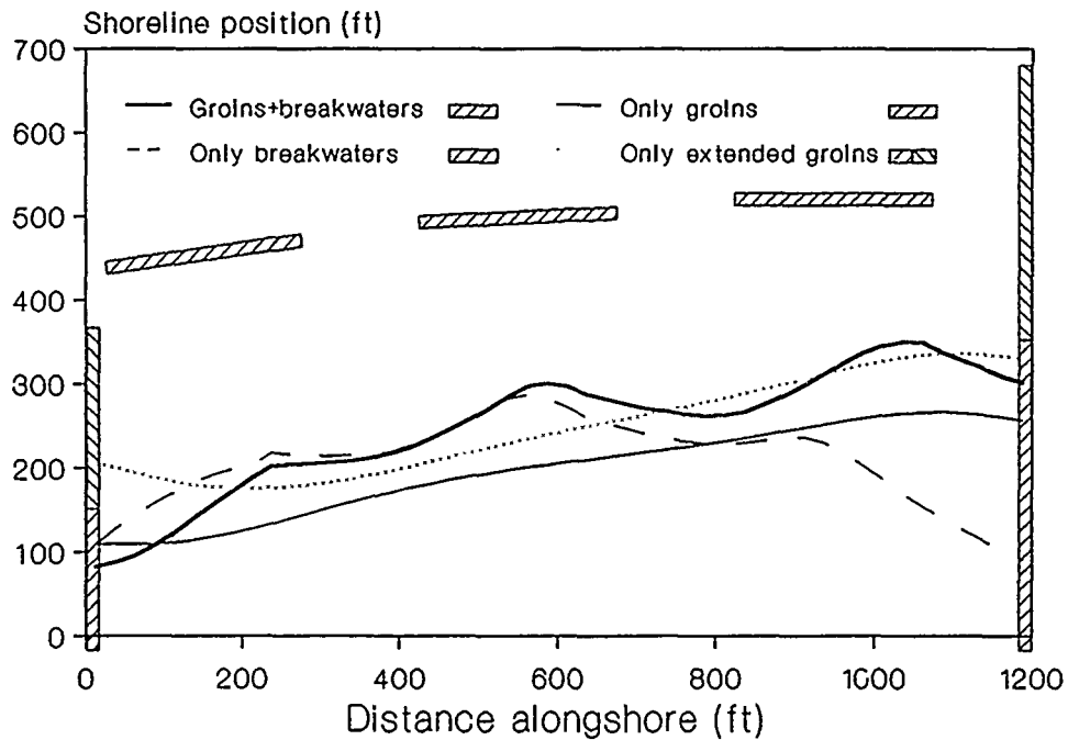
Figure 46. Shoreline change for alternative configurations
